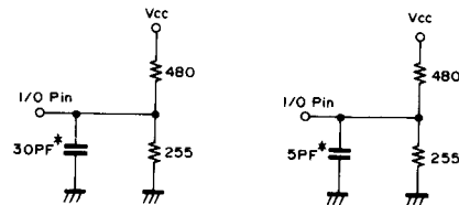
Output Load (2)**
